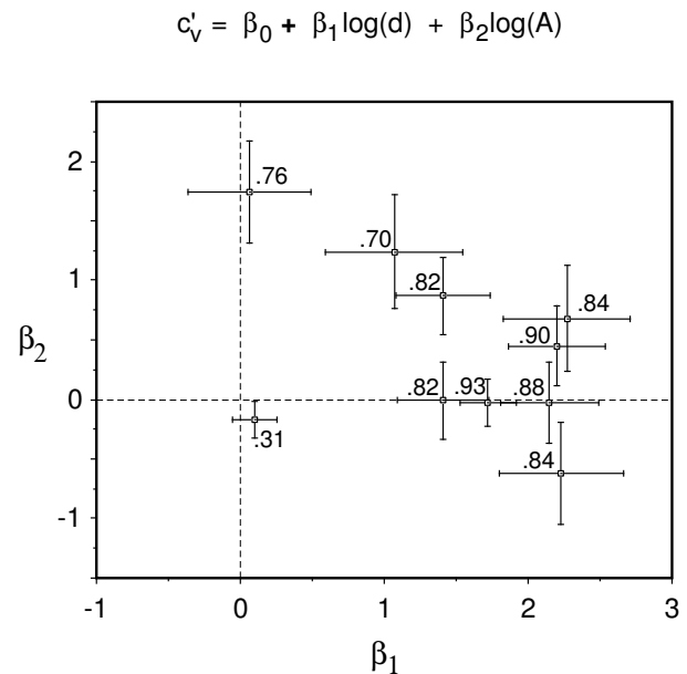
Figure 36. Plot of the coefficients \beta_1 and \beta_2 for the linear model, c'_v = \beta_0 + \beta_1 \log(d) + \beta_2 \log(A) in Experiment 5. Each point represents a different subject. Also shown are 95% confidence intervals, and r^2 -values for the model.
