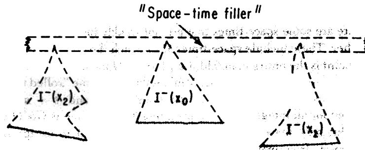
Figure 4. "Clothesline construction" by which a space-time is formed in which all the past observation sets I^-(x_i) can be isometrically embedded.
