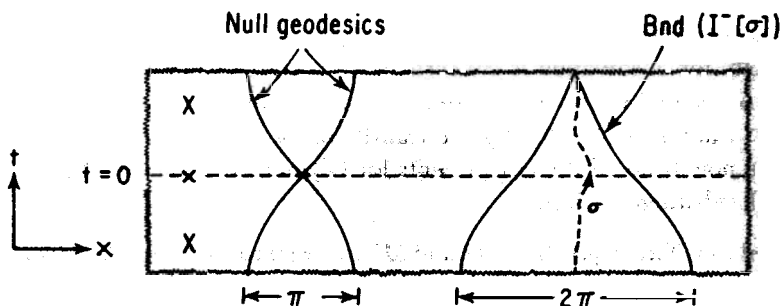
Figure 1. The covering space of two-dimensional De Sitter space-time, i.e., the t, x plane with metric ds^2 = dt^2 - (\cosh^2 t) dx^2 . Light cones narrow rapidly to the vertical as |t| \rightarrow \infty . Every future-extendible timelike curve \sigma has an observational horizon of x -width 2\pi . Two-dimensional De Sitter space-time arises by identifying all points (t, x + 2n\pi) for integers n . By introducing coordinates \tilde{t} = \sinh t, \tilde{x} = (\cosh t) (\cos x), \tilde{y} = (\cosh t) (\sin x) , it assumes the familiar form of a hyperboloid of one sheet -\tilde{t}^2 + \tilde{x}^2 + \tilde{y}^2 = 1 in \mathbb{R}^3 with metric ds^2 = -d\tilde{t}^2 + d\tilde{x}^2 + d\tilde{y}^2 .
