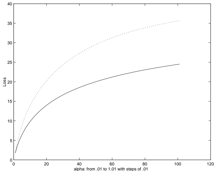
Figure 1: Plot of the loss against \alpha in RPE (dotted line) and REE (solid line).
