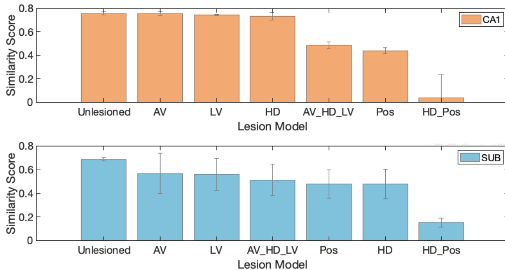
Fig. 8: Ablation studies: similarity scores of the unlesioned and lesioned models. Bars show the mean values and the error bars show standard deviation of scores obtained by 5 instances of each model. Lesions of the positional input (Pos) in the CA1 model had the strongest impact on the network performance compared to lesions of other single input streams. In the SUB model, lesions of all four types of input had a similar level of impact on the network performance.
