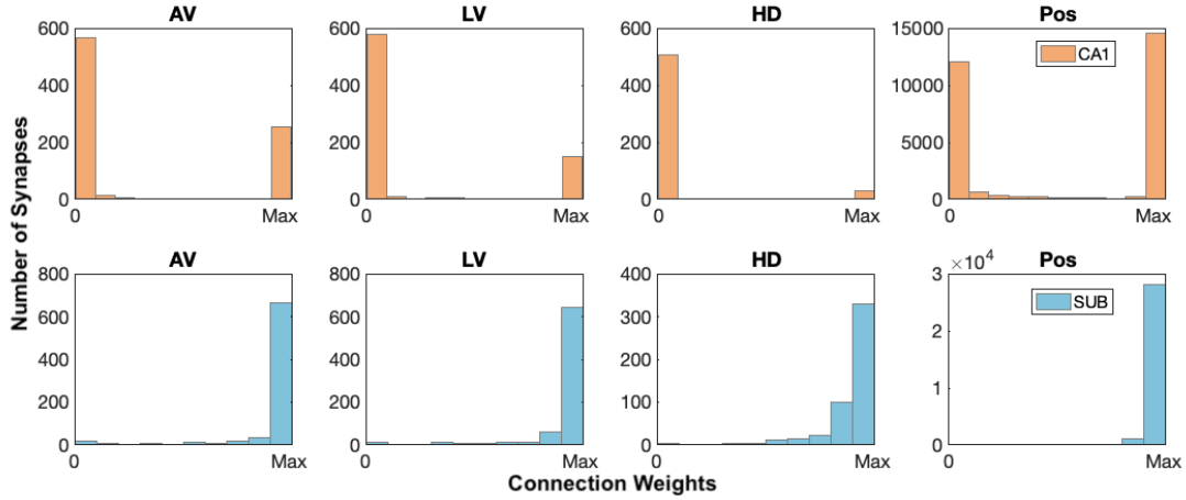
Fig. 5: Histograms of the connection weights from the input groups to the excitatory neuron groups. Weight values range from 0 to the maximum weight value, which was evolved by the EA. CA1 weights show more weights near 0 for AV, LV, and HD, and more weights near the maximum weight for Pos. In the SUB model, weight values of all four types of input all cluster near the maximum weight value.
