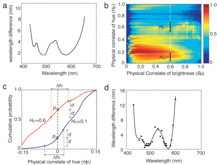
Fig. 1. Statistical explanation of the hue discrimination function. (a) The wavelength change in a monochromatic stimulus needed to elicit a just noticeable difference in hue (after ref. 1). (b) Joint probability distribution of the physical correlates of hue and brightness, P(H_p, B_p) , obtained from the image database (probability values in this and subsequent figures are indicated by color coding; see bar on right). (c) Cumulative density functions of P(H_p|B_p) at two different values of the physical correlate of hue ( H_{p1} = 0.6 , H_{p2} = 0.1 ) for the same physical correlate of brightness ( B_p = 0.6 ), obtained by normalizing and accumulating the probability values of P(H_p|B_p) within a local window. The abscissa shows the relative value of the physical correlate of hue with respect to the center of the local window. (d) The predicted changes in wavelength needed to maintain constant perceived differences in hue. The points are the constant differences in cumulative density functions at the indicated wavelengths, using 0.02 as a value for d (the scale of d in c has been enlarged for clarity); the solid curve is a polynomial fit.
