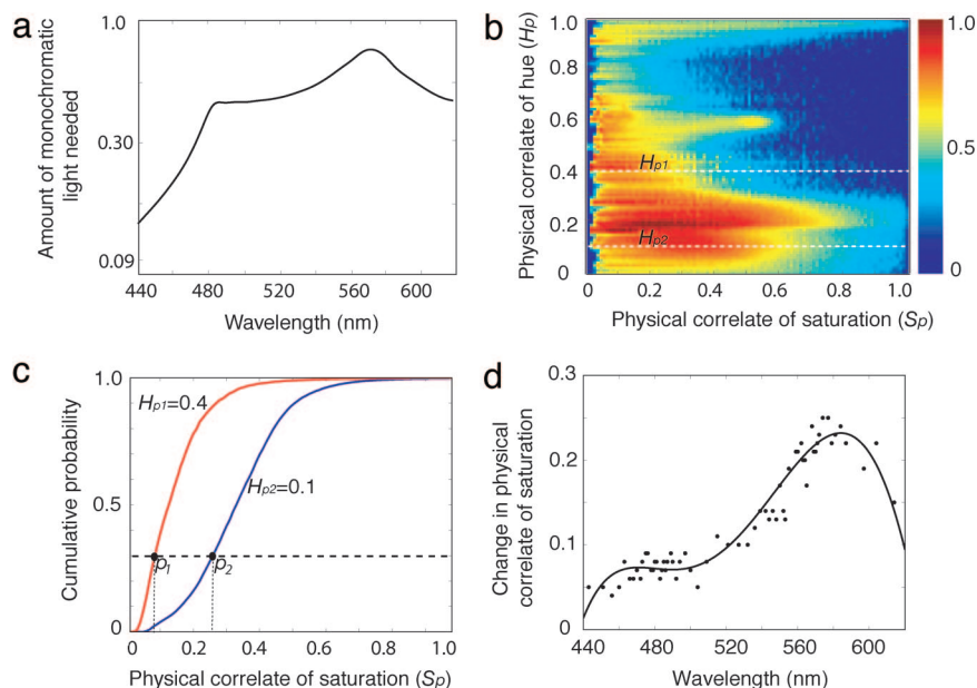
Fig. 2. Statistical explanation of the saturation discrimination function. (a) The amount of monochromatic light needed to generate the same perceived saturation difference with respect to neutral gray at different wavelengths (after ref. 2). (b) Joint probability distribution of the physical correlates of hue and saturation, P(H_p|S_p) , obtained from the image database. (c) The cumulative density functions of P(S_p|H_p) when the physical correlate of hue was 0.1 (blue curve; \approx 575 nm) or 0.4 (red curve; \approx 515 nm). (d) The predicted changes in the physical correlates of saturation needed to maintain a constant difference in perceived saturation as a function of the wavelength (the value illustrated is 0.3 in the cumulative density function, as shown in c). The points were derived from the cumulative density functions at the indicated wavelengths; the solid curve is a polynomial fit.
