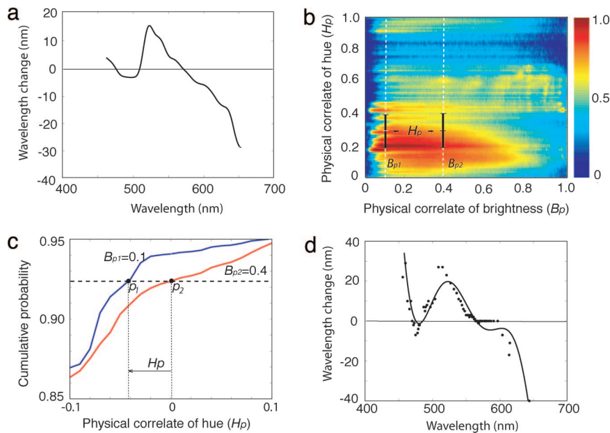
Fig. 5. Statistical explanation of the Bezold–Brücke effect. (a) Psychophysical data showing the changes in wavelength needed to match the hue of a monochromatic light presented at a higher intensity (after ref. 6). (b) Joint probability distribution of the physical correlates of hue and brightness, P(H_p, B_p) , obtained from the database. (c) The cumulative density functions of P(H_p|B_p) calculated within a \pm 0.1 window centered at 0.3 as the value of the physical correlate of hue, given a lower and a higher levels of the physical correlate of brightness (indicated by the dashed lines in b). (d) The predicted hue shifts for the indicated points; the solid line is a polynomial fit.
