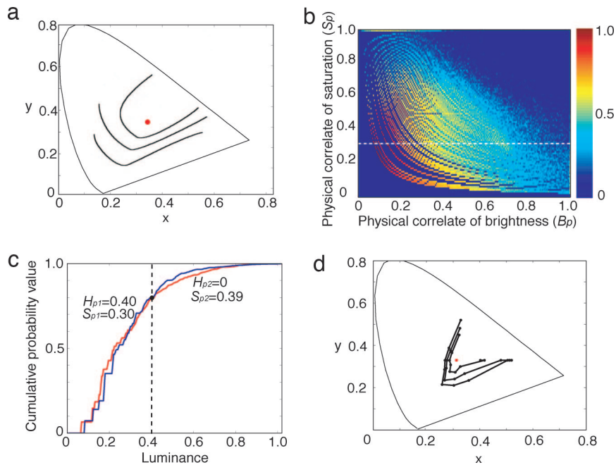
Fig. 6. Statistical explanation of the Helmholtz-Kohlrausch effect. (a) Psychophysical changes in brightness as a function of both hue and saturation, plotted in the 1931 CIE chromaticity diagram (after ref. 8; the red dot indicates the white point). (b) Joint probability distribution of the physical correlates of saturation and brightness, P(S_p, B_p) , at a particular value of the physical correlate of hue ( H_p = 0.1 ). (c) The cumulative density functions of the physical correlate of brightness when the physical correlate of saturation is 0.3 and the physical correlate of hue 0.4 (blue curve) and when the physical correlate of saturation is 0.39 and the physical correlate of hue 0 (red curve). The cumulative probability values in these functions at a physical correlate of brightness value of 0.4 are the same. (d) The equal-brightness curves predicted by these statistics. Each of the points on a given curve has the same physical correlate of brightness value (0.2) and the same predicted brightness. The relative closeness of these curves reflects the limited number of highly saturated samples in the database and the limited gamut of the xy values in the CIE chromaticity diagram that can be represented by RGB values.
