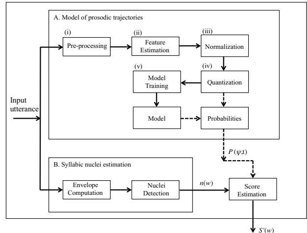
Figure 1: Overview of the processing steps in the algorithm.
