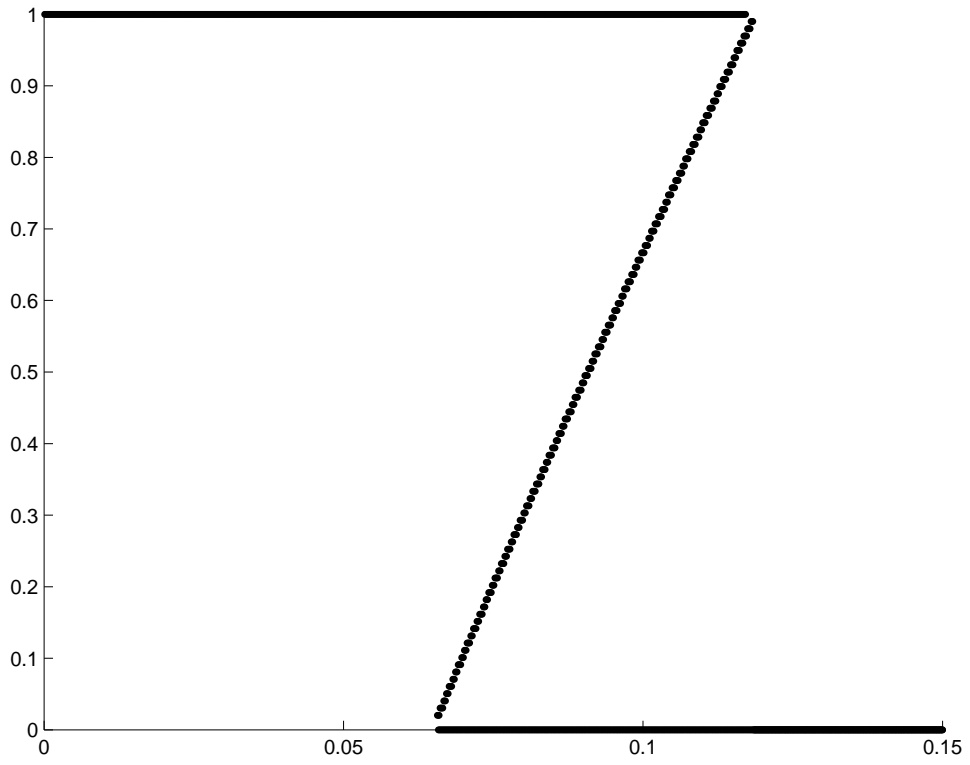
Figure 2: Bifurcation Diagram.
