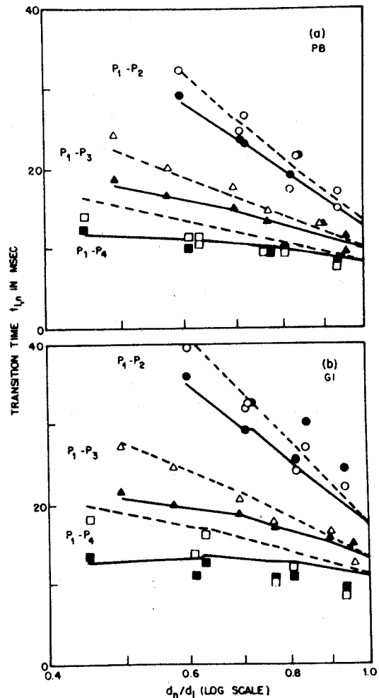
Figure 7. Predicted transition times for the modified model. (Experiment 2 data are replotted as in Figure 3. The predicted transition times based on Equation 12 are joined by solid curves for the 2-m viewing distance and dashed curves for the 1-m distance.)
